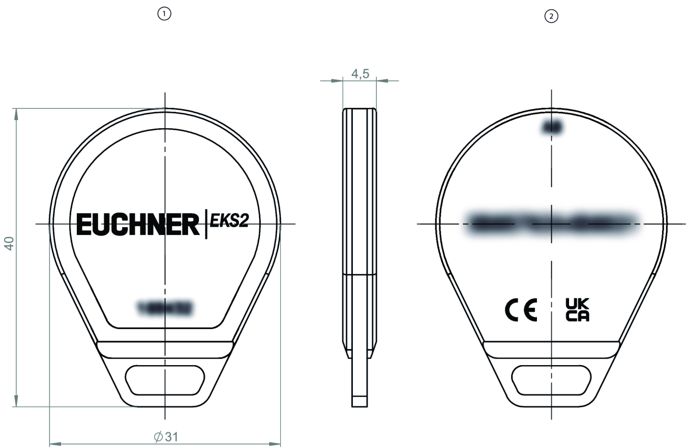
1 Front view
